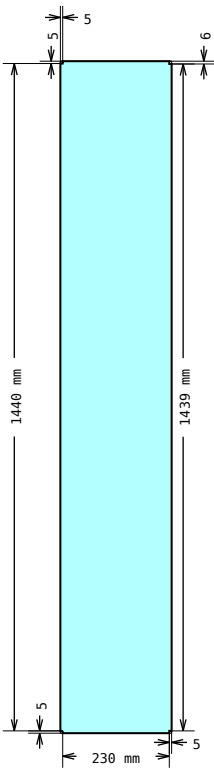
DRAWING 4, Pos 16 Shape measurements
