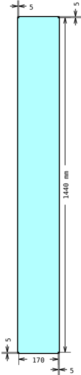
DRAWING 3, Pos 15 Shape measurements
