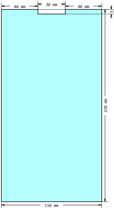
DRAWING 2, Pos 14 Shape measurements
